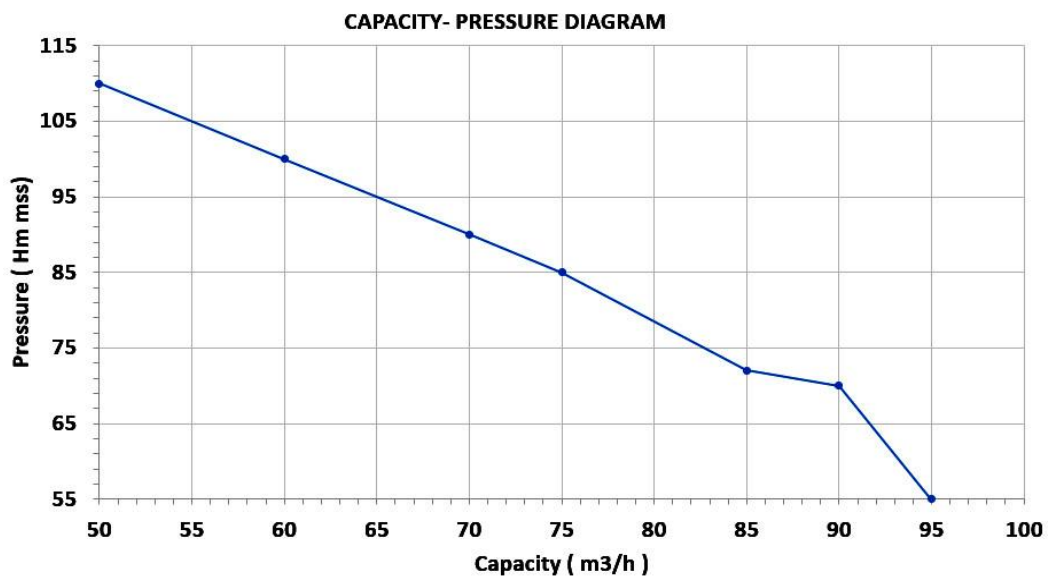
P014- 45D - KP65B3/50 P015 - 45 HP Diesel Motopump Water Cooler - 4 Cylinders 3 Stage High Pressure with Trailer List Price= 39,861,000 TSH Suction 4" - Outlet 4"
