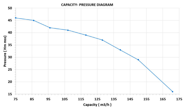
P036-25 HP Electric Motorpump - 3 Cylinder - 1 Stage High Volume Suction 5" - Outlet 4"
