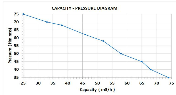
P013- 22D - KP500B2/20 22HP Diesel Motopump Water Cooler - 3 Cylinders - 2 Stage List Price= 25,230,000 TSH Suction 4" - Outlet 4"
