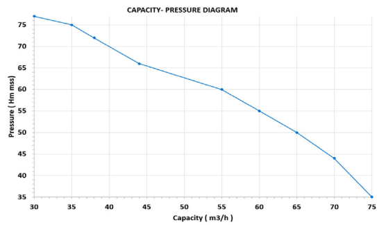
P037-20 HP Electric Motorpump - 3 Cylinder - 2 Stage High Pressure Suction 3" - Outlet 2,5"
