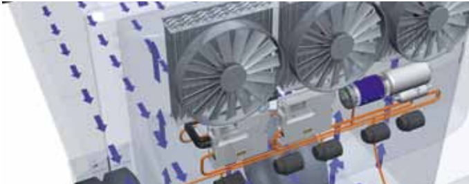
DCU: Refrigerator trailer – compressors and fans
