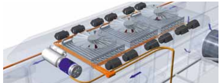
DCU/PSU: Controlling the compressor and the ventilation system
