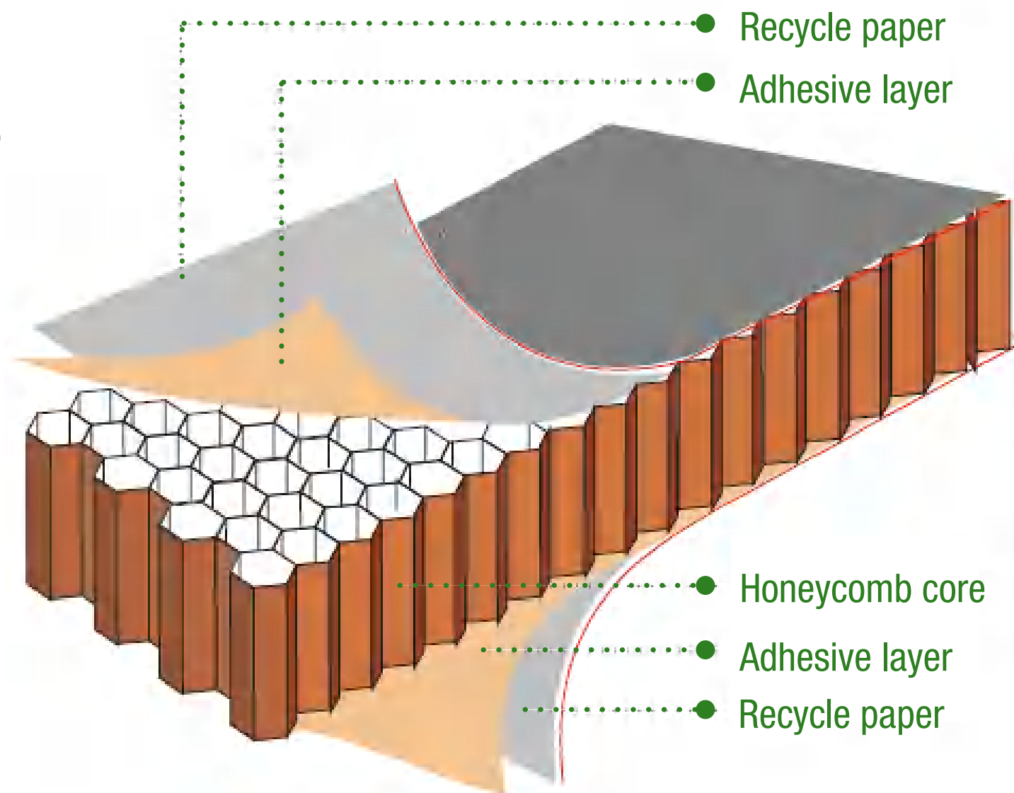
Composite Paper Honeycomb Core Material Details
